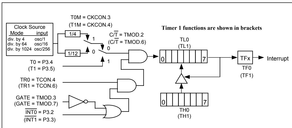
Figure 12. Timer/Counter Mode 2.
