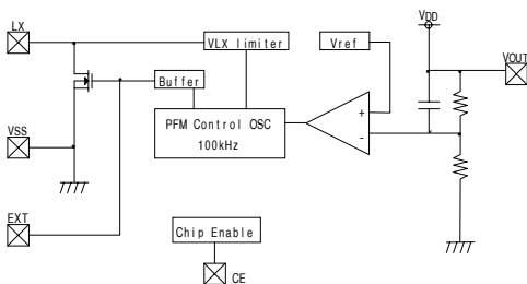
(1) XC6382A~XC6382D(VOUT端与VDD兼用)
