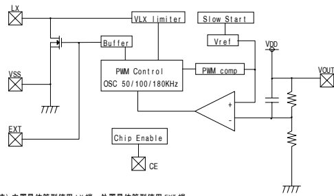
(1) XC6372A~XC6372D (VOUT端与VDD兼用)
