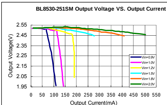
3.Output Voltage VS. Output Current
