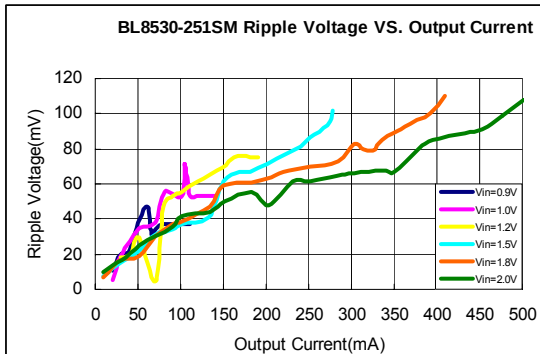
7.Ripple VS. Output Current
