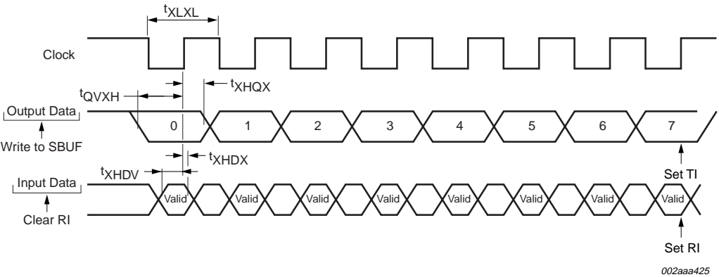
Fig 11. Shift register mode timing.
