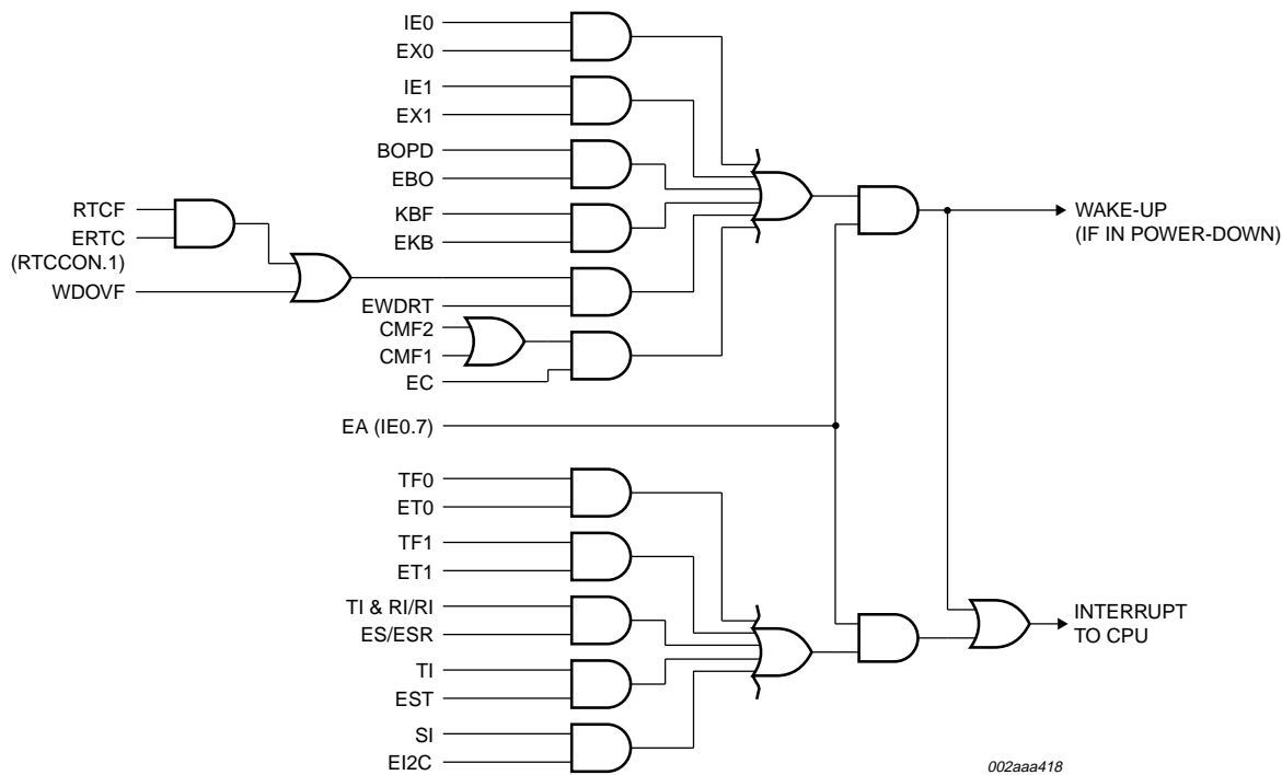
Fig 5. Interrupt sources, interrupt enables, and power-down wake-up sources.
