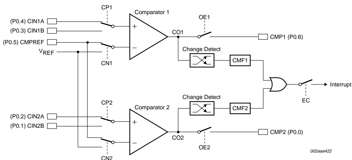
Fig 9. Comparator input and output connections.
