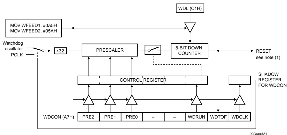
Fig 10. Watchdog timer in watchdog mode (WDTE = '1').
