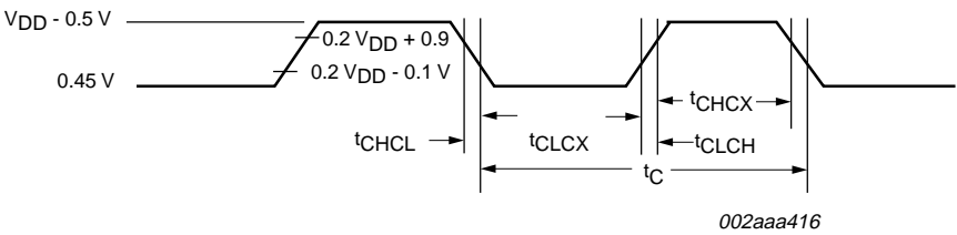
Fig 12. External clock timing.
