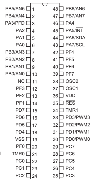
HT46R24/HT46C24 48 SSOP-A
