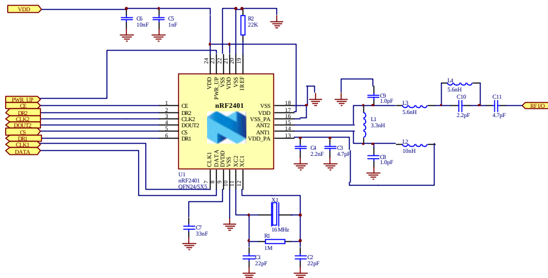
Figure 21 nRF2401 schematic for RF layouts with single end 50Ω antenna
